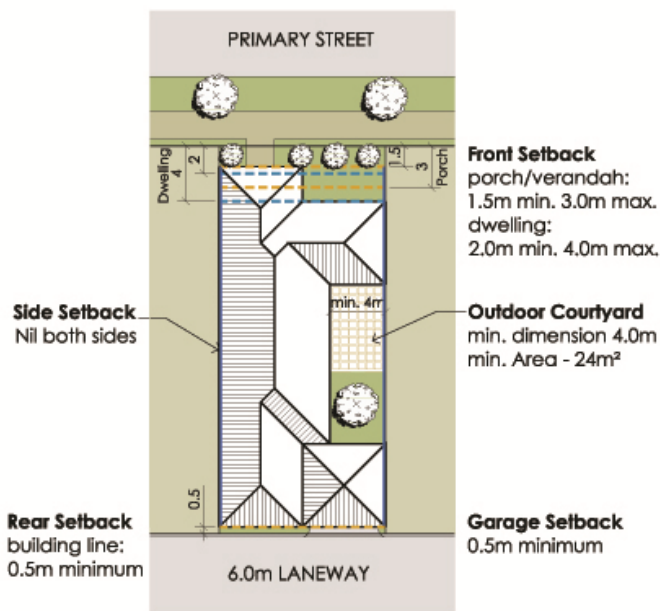
Cottage Lot (R40/R60) setbacks when access from rear laneway
