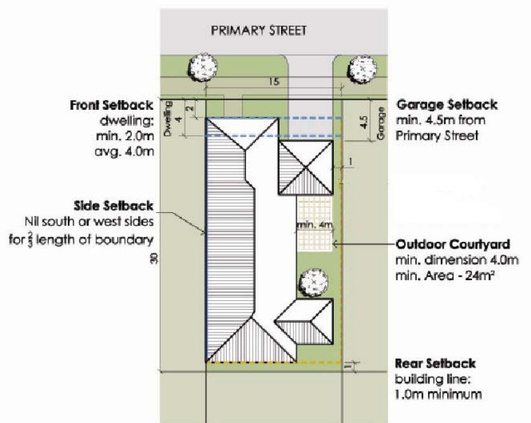
Traditional Lot (R30) setbacks when access from front
