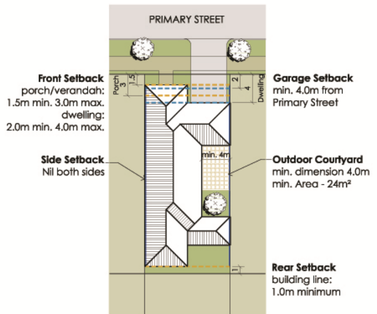
Cottage Lot (R40/R60) setbacks when access from front
