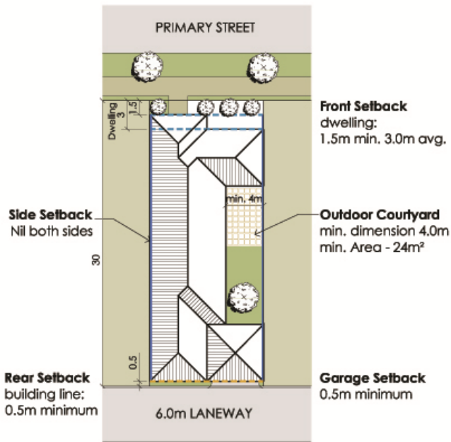
Traditional Lot (R30) setbacks when access from rear laneway
